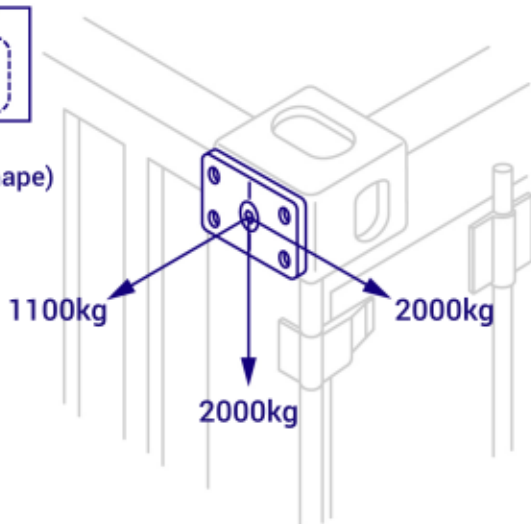
Top end holes (Shield Shape)
